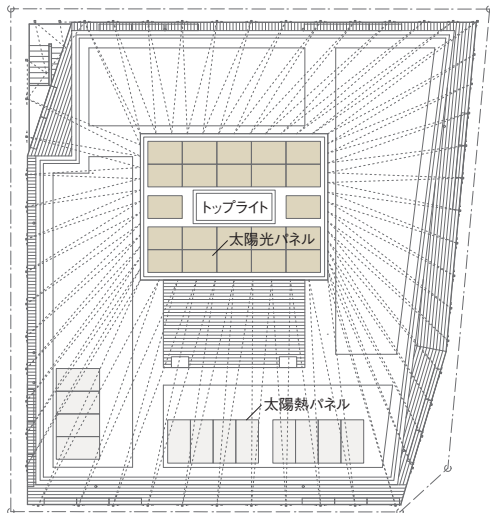
Roof plan
